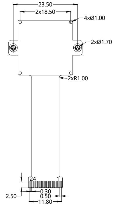
BOTTOM VIEW
